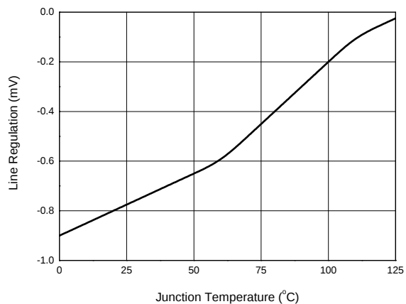
Line Regulation vs. Junction Temperature
